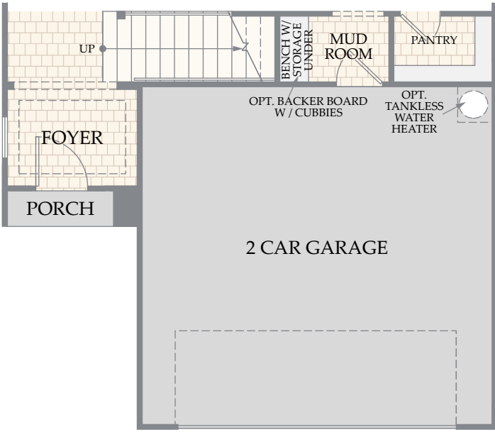
ELEVATION B AT MAIN LEVEL
