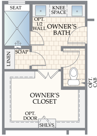
OPTIONAL ENLARGED CLOSET SHOWER at OWNER'S BATH AT SECOND LEVEL
