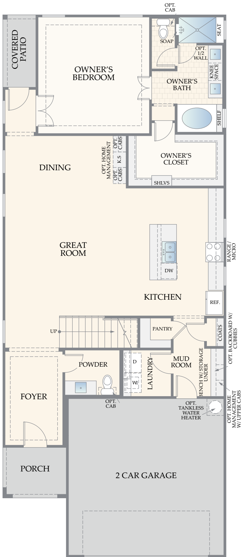
MAIN LEVEL LAGUNA PLAN 301
