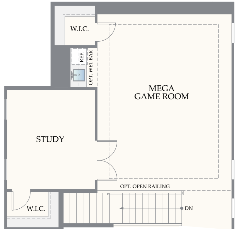
OPT. STUDY w/ MEGA GAME ROOM ILO BEDROOM 4 AT SECOND LEVEL
