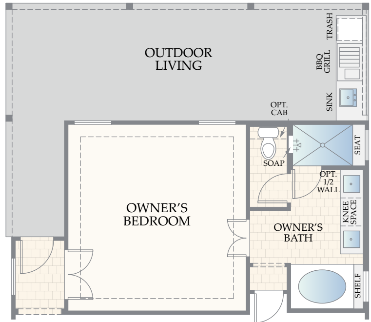
OPT. OUTDOOR LIVING w/ KITCHEN AT MAIN LEVEL
