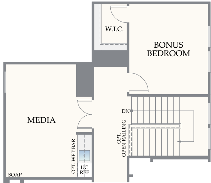
OPTIONAL BONUS BEDROOM / CLOSET & MEDIA I.L.O. BEDROOM 2 AT SECOND LEVEL
